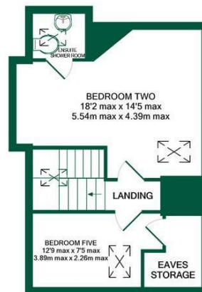
SECOND FLOOR APPROX. FLOOR AREA 416 SQ.FT. (38.6 SQ.M.)
